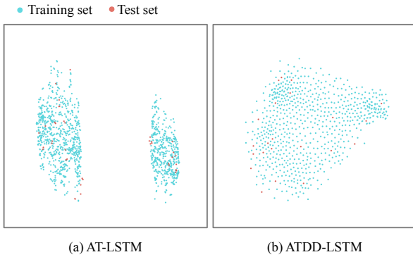
Figure 6. Visualization of feature embedding using t-SNE on the training (source) set and test (target) set of DEAP. (a) shows the feature space of using AT-LSTM (the method without the domain discriminator). (b) shows the feature space of using ATDD-LSTM.
